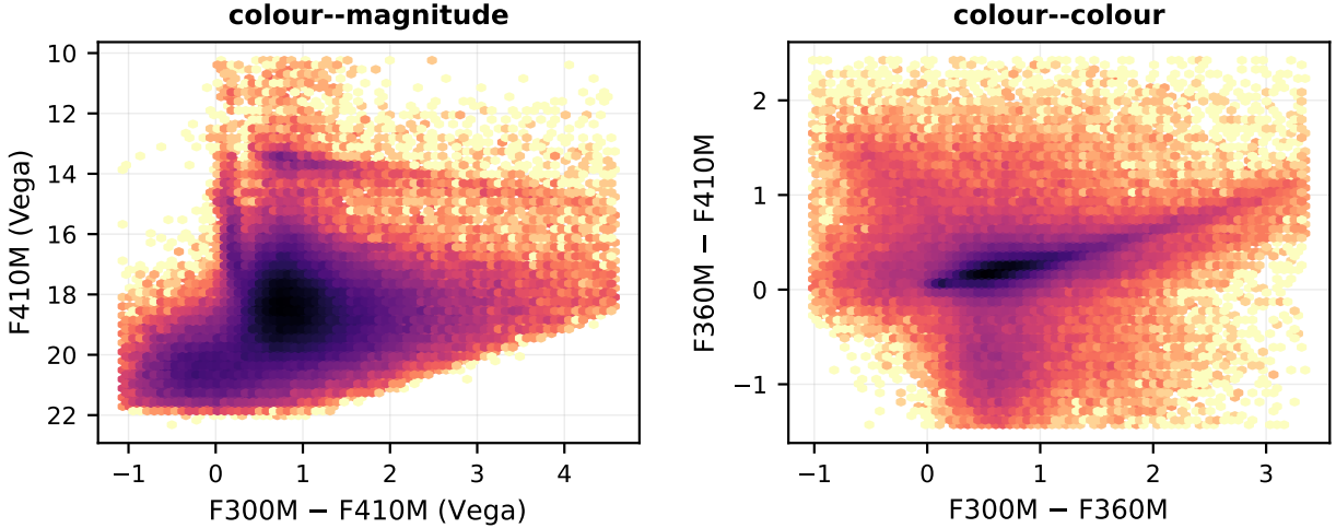
Figure 6: Colour diagrams for sgrb2, from the stage-m7 cross-band merge, in Vega magnitudes. These are differential between filters and so respond to systematics that per-filter statistics cannot see: a zero-point error shifts a sequence bodily, a saturation-correction discontinuity breaks it at a specific magnitude, and a filter-dependent background error tilts it.
