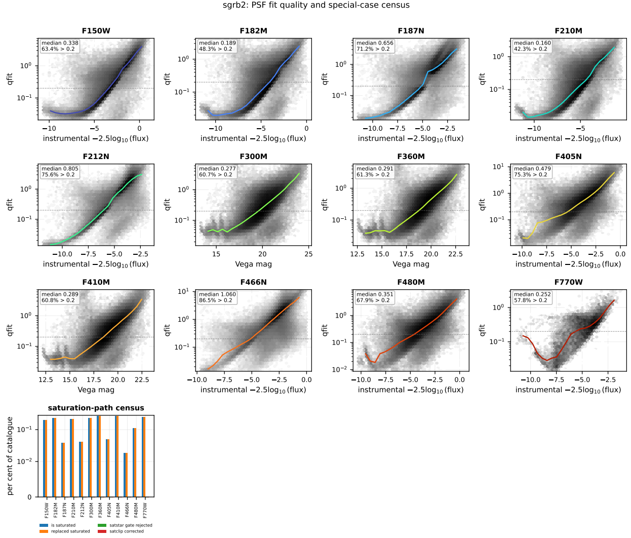
Figure 5: PSF-fit quality for sgrb2. Per filter, the normalised fit residual q_{\text{fit}} against brightness (greyscale: source density; line: running median; dotted: the q_{\text{fit}} = 0.2 vetting threshold). The final panel is the fraction of each filter's catalogue touched by the saturation-handling paths: flagged saturated, core-replaced, rejected by the saturated-star gate, and clip-corrected.
