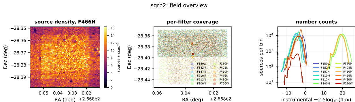
Figure 1: Overview of sgrb2. Left: source surface density in 72 \times 72 sky cells for F466N, the filter with the most detections. Centre: the sky coverage of each filter, sub-sampled. Right: number counts per filter; the peak of each curve is the turnover magnitude, the practical completeness limit beyond which the counts are set by detectability rather than by the stellar population.
