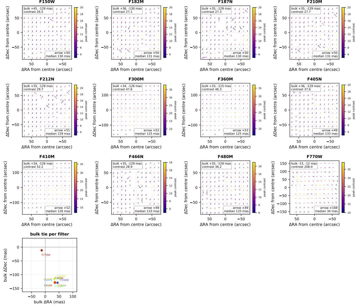
Figure 3: Absolute astrometry of sgrb2 against its registered reference catalogue. Each per-filter panel maps the offset-histogram tie on a 12 \times 12 tile grid (arrows, exaggerated; colour is the per-tile peak contrast), with the whole-field bulk tie quoted in the corner. Grey crosses mark tiles whose tie was only found by widening the search window and whose offset is therefore not trustworthy. The final panel collects the bulk ties. Offsets are measured by offset-histogram stacking, which is immune to the nearest-neighbour pairing collapse that a median against a dense reference suffers; the per-tile map is shown because a bulk offset near zero does not by itself mean the field is registered.
