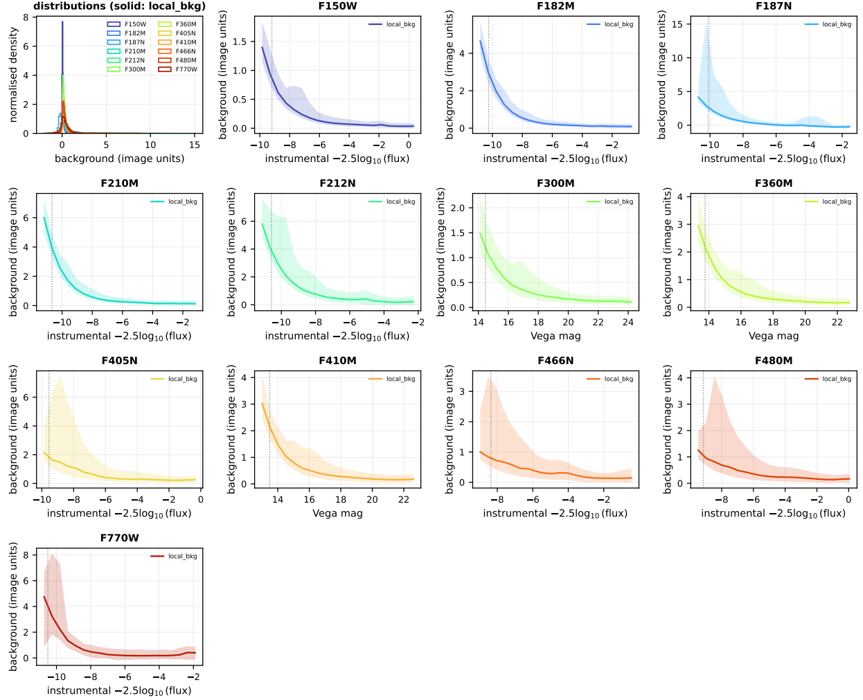
Figure 7: Background estimators for sgrb2. First panel: the distribution of the annulus background handed to the fitter (solid) and, where available, the residual-footprint background (dashed). Remaining panels: the running median of each against brightness, with the 16–84th percentile band for the annulus estimator; the vertical dotted line marks the brightest 1 per cent, where a star’s own wings begin to enter its own background aperture. The residual-footprint column is present for 0 of 12 filters; it was added in 2026-07, so catalogues produced before then carry only the annulus estimator.
