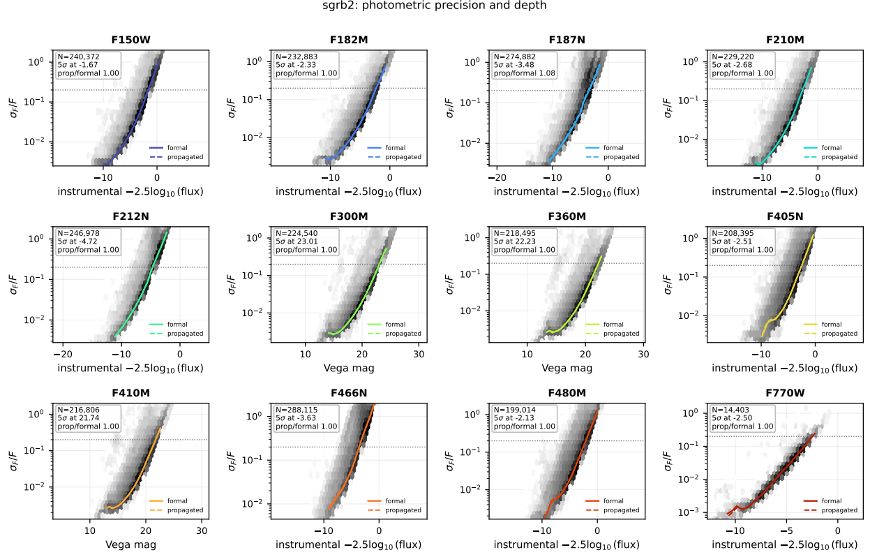
Figure 4: Photometric precision of sgrb2. Greyscale is source density; the solid line is the running median of the fitter’s formal uncertainty \sigma_F/F and the dashed line the same quantity propagated from the per-exposure scatter. The dotted horizontal line is \sigma_F/F = 0.2 , and where the median crosses it is quoted as the 5\sigma depth. A propagated-to-formal ratio above unity means the exposures disagree by more than the fit covariance predicts.
