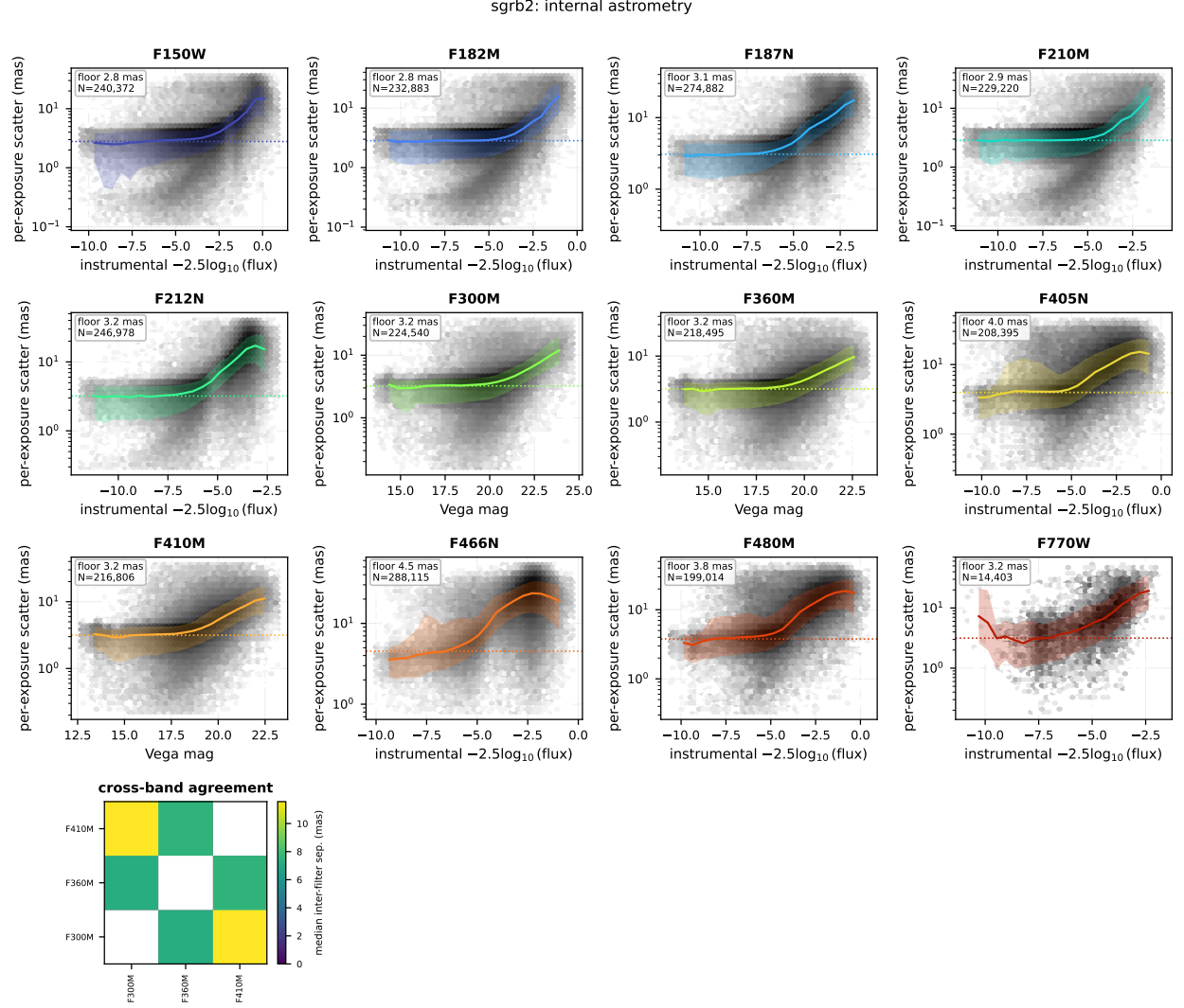
Figure 2: Internal astrometry of sgrb2. Per filter: the scatter of the individual-exposure centroids about the merged position, against brightness; greyscale is source density, the coloured line and band are the running median and 16–84th percentile, and the dotted line marks the bright-decile floor quoted in the panel. The final panel is the median separation between the same stars measured independently in each pair of filters; only sources independently detected in both bands are counted, since a forced or seeded position imported from another band would measure the merge radius rather than the astrometry.
